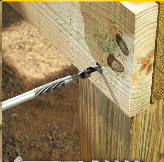
AUGERBOLT™ THROUGH BOLT FASTENING
